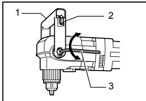
1. Spade grip 2. Wrench holder 3. Hex wrench
