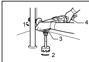
1. Reaction 2. Forward 3. Spade grip 4. Handle
