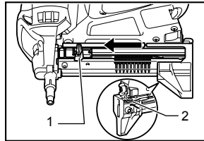
1. Pusher lever 2. Nail stopper
