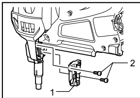
1. Under driver guide 2. Bolt
