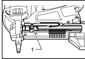
1. Pusher lever
