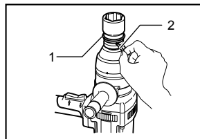
1. O-ring 2. Pin
